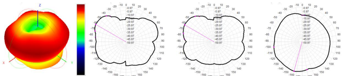
1880M 3D-E1-E2-H
